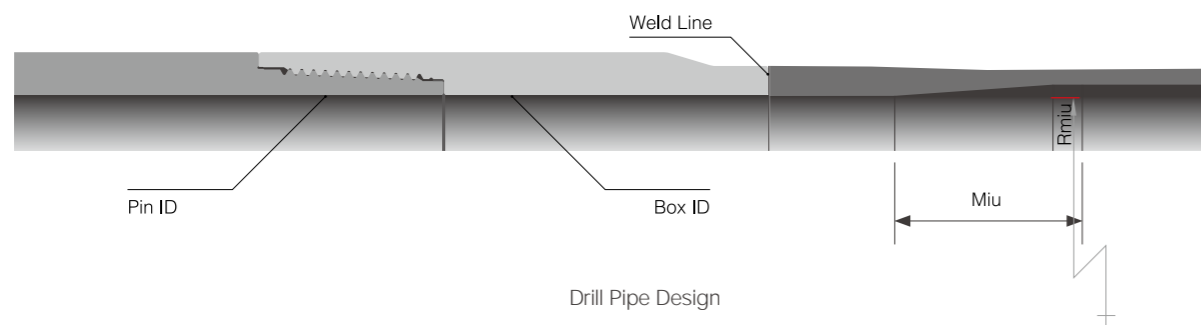
Upset Profile and MIU Control
